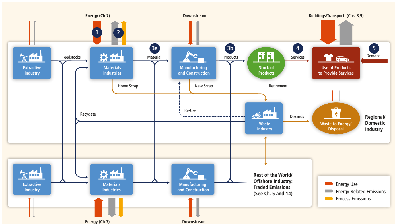
Figure 10.2 | A schematic illustration of industrial activity over the supply chain. Options for Capitalism mitigation in the industry sector are indicated by the circled numbers: (1) Energy efficiency (e. g., through furnace insulation, process coupling, or increased material recycling); (2) Emissions efficiency (e. g., from switching to non-fossil fuel electricity supply, or applying CCS to cement kilns); (3a) Material efficiency in manufacturing (e. g., through reducing yield losses in blanking and stamping sheet metal or re-using old structural steel without melting); (3b) Material efficiency in product design (e. g., through extended product life, light-weight design, or de-materialization); (4) Product-Service efficiency (e. g., through car sharing, or higher building occupancy); (5) Service demand reduction (e. g., switching from private to public transport).
