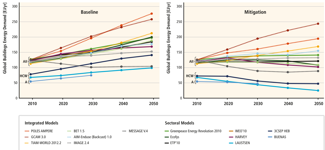
Figure 9.20 | Annual global final energy demand development in the building sector by 2050 (except WEO'10 and BUENAS) in selected sectoral models for baseline (left) and advanced (right) scenarios, for total energy (All, heating/cooling/hot water/lighting/appliances), thermal energy (HCW, includes heating/cooling/hot water), and appliances (A); compared to selected integrated models. Dashed lines show integrated models, solid lines show sectoral/bottom-up models. Sources: Cornelissen et al. (2012), Deng et al. (2012a), Dowling et al. (2012), GPI (2010), Harvey (2010), IEA (2012c0a), Laustsen (2010), McNeil et al. (2013), Üрге-Vorsatz et al. (2012a3), WBCSD (2009), WEO (2011) and WG III AR5 Scenario Database (Annex II.10).
