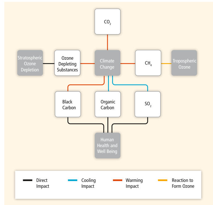
Figure 5.21 | Impacts of and links between selected substances emitted to the atmosphere. Adopted from (UNEP, 2012).
