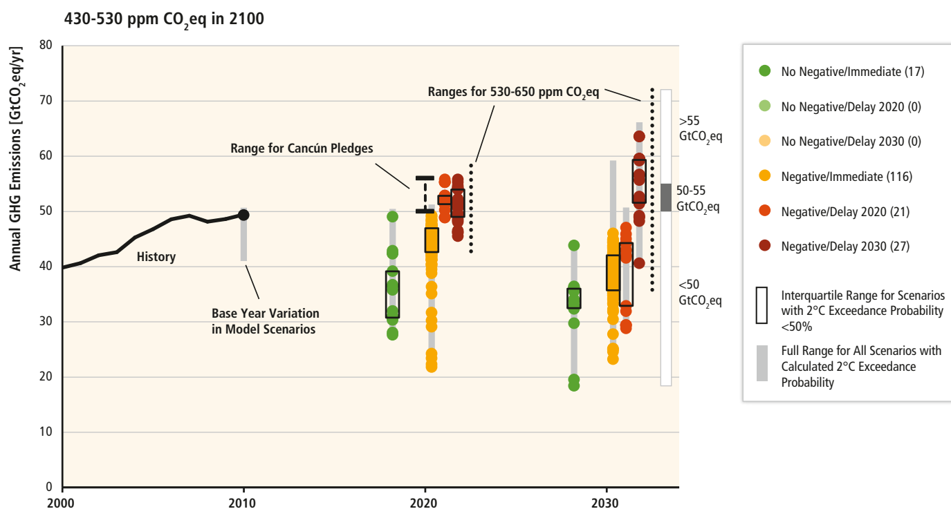
Figure TS.11 | Near-term GHG emissions from mitigation scenarios reaching about 450 to about 500 (430–530) ppm CO 2 eq concentrations by 2100. The Figure includes only scenarios for which temperature exceedance probabilities were calculated. Individual model results are indicated with a data point when 2 °C exceedance probability is below 50 % as assessed by a simple carbon cycle/climate model (MAGICC). Colours refer to scenario classification in terms of whether net CO 2 emissions become negative before 2100 (negative vs. no negative) and the timing of international participation in climate mitigation (immediate vs. delay until 2020 vs. delay until 2030). Number of reported individual results is shown in legend. The range of global GHG emissions in 2020 implied by the Cancún Pledges is based on analysis of alternative interpretations of national pledges. Note: In the WGIII AR5 scenario database, only four reported scenarios were produced based on delayed mitigation without net negative emissions while still lying below 530 ppm CO 2 eq by 2100. They do not appear in the figure, because the model had insufficient coverage of non-gas species to enable a temperature calculation. Delay in these scenarios extended only to 2020, and their emissions fell in the same range as the ‘No Negative/Immediate’ category. Delay scenarios include both delayed global mitigation and fragmented action scenarios. [Figure 6.31, 13.13.1.3]
