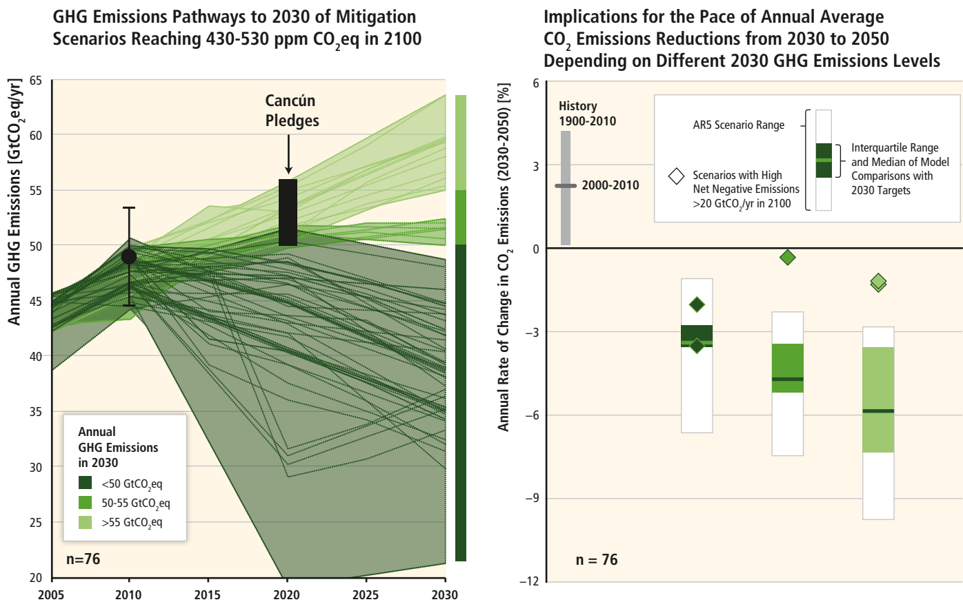
Figure 6.32 | The implications of different 2030 GHG emissions levels for the pace of CO 2 emissions reductions to 2050 in mitigation scenarios reaching 430–530 ppm CO 2 e by 2100. Left-hand panel shows the development of GHG emissions to 2030. Right-hand panel denotes the corresponding annual CO 2 emissions reduction rates for the period 2030–2050. The scenarios are grouped according to different emissions levels by 2030 (colored in dark, medium and light green). The range of global GHG emissions in 2020 implied by the Cancún Pledges is based on an analysis of alternative interpretations of national pledges (see Section 13.13.1.3 for details). The right-hand panel compares the median and interquartile range across scenarios from recent intermodelling comparisons with explicit 2030 interim goals with the range of scenarios in the WG III AR5 Scenario Database (Annex II.10). Extreme scenarios with very high net negative emissions (>20 GtCO 2 /yr) in 2100 are reported separately as diamonds. Annual rates of historical emissions change between 1900-2010 (sustained over a period of 20 years) and average annual emissions change between 2000-2010 are shown in grey. Sources: Intermodelling comparisons with explicit interim goals (AMPERE: Riahi et al., 2013; LIMITS: Kriegler et al., 2013b; ROSE: Luderer et al., 2013) and the WG III AR5 Scenario Database (Annex II.10). Historic data: JRC/PBL (2013), IEA (2012a), see Annex II.9. Note: Only scenarios with default technology assumptions are shown. Scenarios with non-optimal timing of mitigation due to exogenous carbon price trajectories are excluded.
